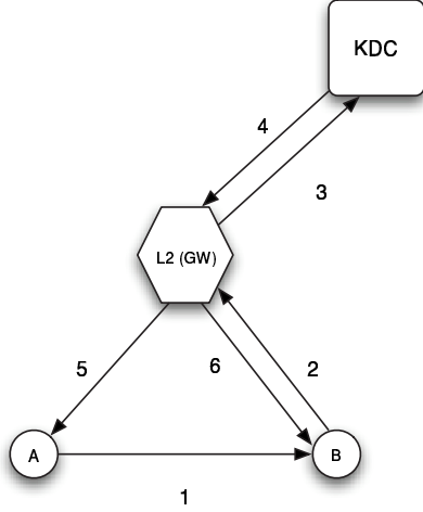
Fig. 4. The message flow for key establishment in the LIGER system. Node A sends a token to Node B indicating its desire to establish a session key. B includes its own token and forwards that message to the KDC via the gateway. The KDC determines the validity of both tokens and returns a message to the L2 containing a copy of a session key encrypted in a new, randomly chosen authenticator key for both A and B . The message from the KDC will also contain a bitmap corresponding to each of the authenticator keys used to sign the session keys. Nodes A and B then receive a transmission from the L2 node, generate the appropriate authenticator keys to unlock the session key and begin communication. The messages for this protocol flow as shown in Figure 4 and appear as follows.
