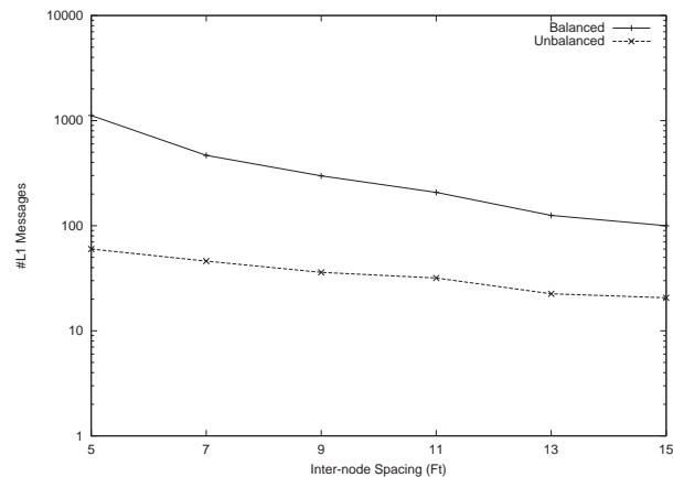
Fig. 10. The average number of messages per L1 node to initialize networks with varying inter-node spacing.
