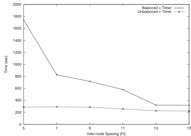
Fig. 8. Balanced and Unbalanced network initialization times for the LION scheme with varying inter-node spacing.
