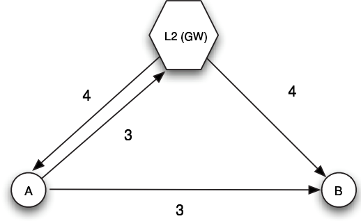
Fig. 2. The Indirect phase of the LION protocol. After node A is unable to establish keys with all of its neighbors, it launches a “Request for Assistance” message. The L2, overhearing this request, provides a session key to both parties.
